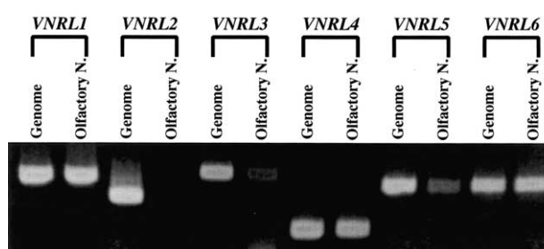
Fig. 1. RT-PCR was performed on mRNA from olfactory nerve tissue of a 36 year old man for putative pheromone receptors. VNRL1 is the same gene as VIRL1 reported previously [19]. The PCR products, amplified from the genome and the olfactory nerve mRNA, have the same size, indicating that these mRNA sequences were not divided by an intron on the genome.
